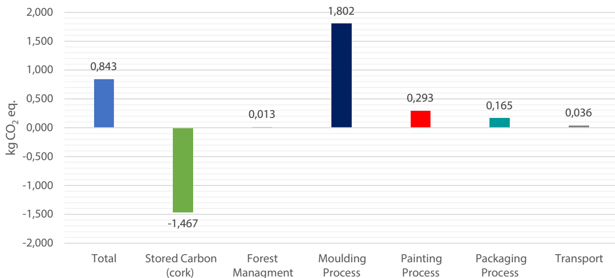
Figure 3: Partial Carbon footprint for the product stage of KORKO | 60pp set – per process stage.
