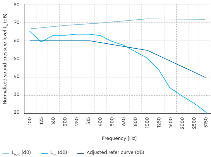
Impact Insulation (IS) · Laminate Floor (8mm) · T85 (2mm) · Floating
