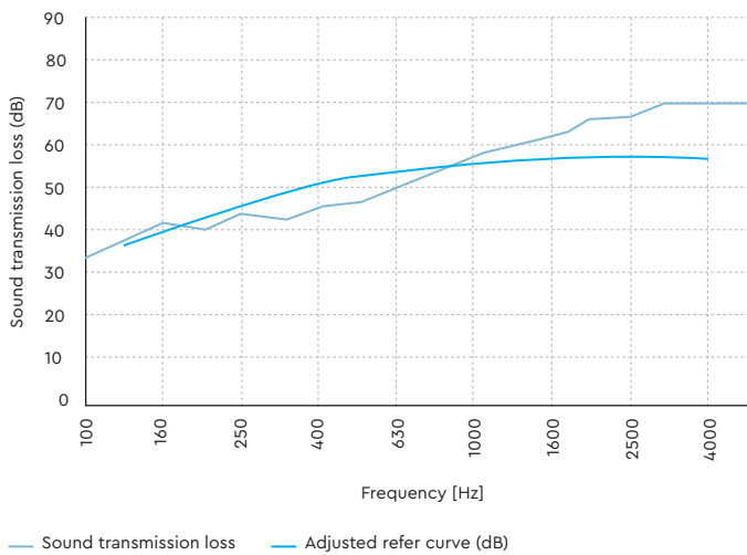
Sound Transmission Class (STC) · Laminate Floor (4mm) · T85 (2mm) · Floating
