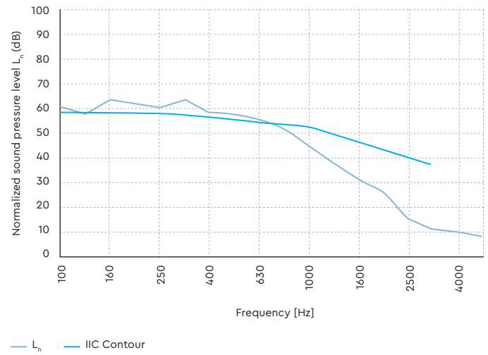
Impact Insulation Class (IIC) · Laminate Floor (4mm) · T85 (2mm) · Floating
